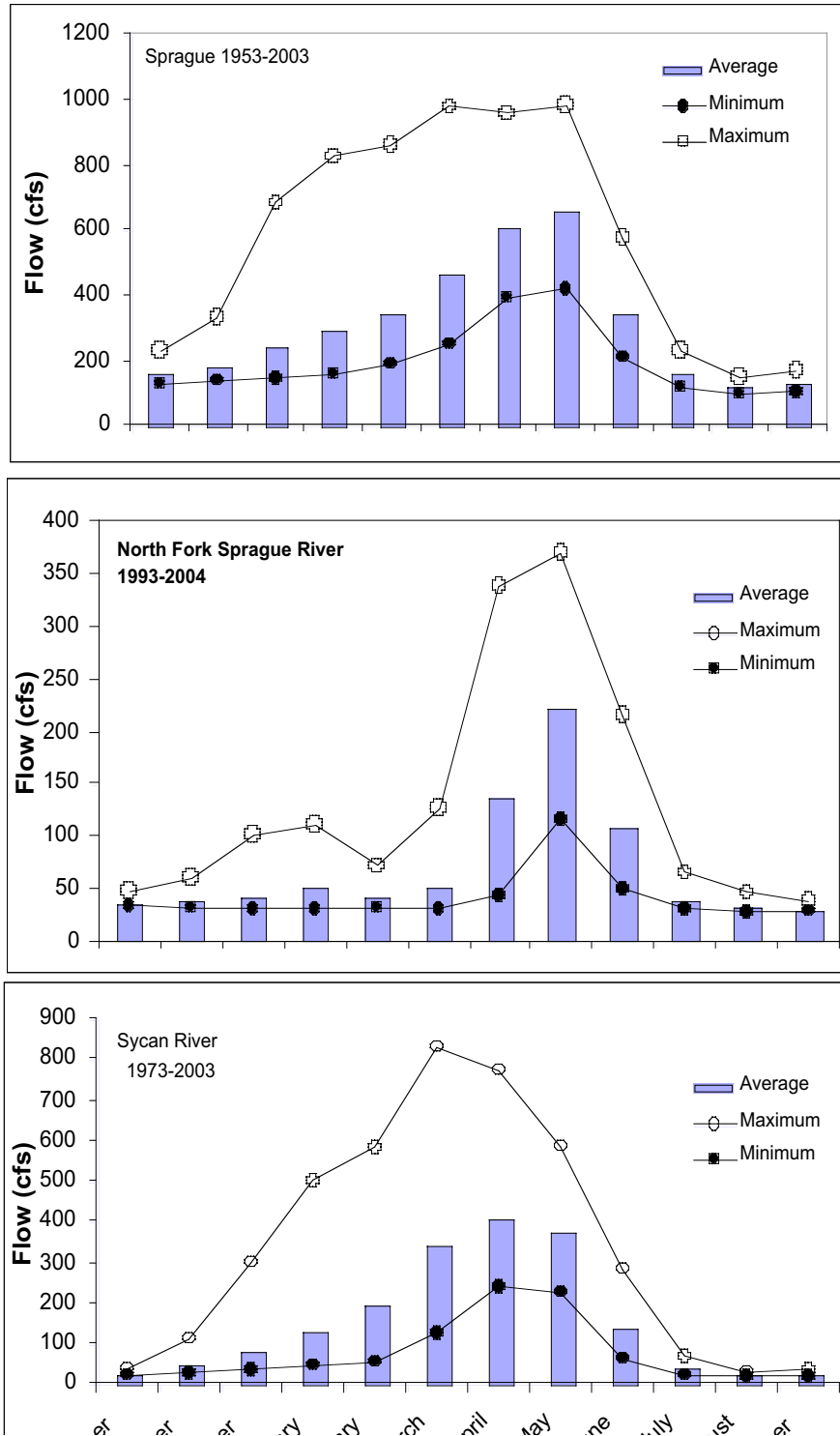
Figure 5-5. Monthly stream flow throughout the period of record in the Sprague River near Beatty (Gage 11497500, top), the North Fork Sprague River at Power Plant (Gage 11495800, center), and the Sycan River below Snake Creek (Gage 11499100, bottom). (Data Source: OWRD 2005)
